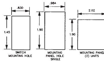
PANEL CUTOUTS
